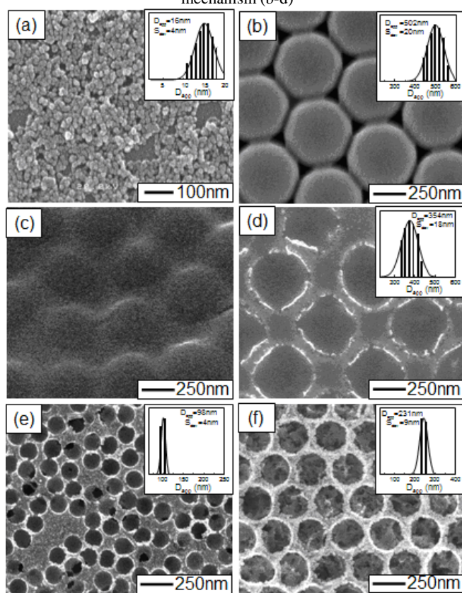
Fig. 2 SEM images of initial colloidal particles (ATO (a) and PS (b)) and coated film before (c) and after template removal process (d-f). using different PS sizes (500 (c and d), 130, and 300 nm (f)). SEM images of coated film using different PS sizes: (c and d) 500, (e) 130, and (f) 300 nm.
