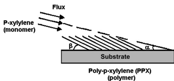
Fig. 1. Schematic of oblique angle deposition combined with pyrolysis of p -xylylene. The deposition process starts with [2.2]paracyclophane dimer and then converted to the poly( p -xylylene) film on a substrate at an oblique angle ( \alpha = 10^\circ ).
