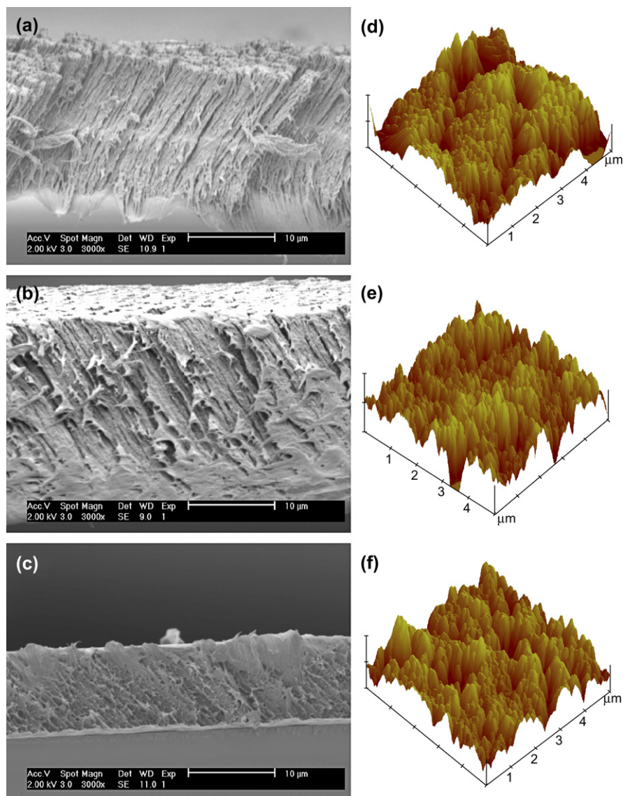
Fig. 3. Cross-sectional SEM images of columnar nanostructured. (a) F-PPX, (b) Cl-PPX, and (c) Br-PPX and corresponding surface images obtained by contact mode-AFM (scale bars for AFM scans: X: 1 \mu\text{m}/\text{div} , Y: 1 \mu\text{m}/\text{div} , Z: 350 nm/div).
