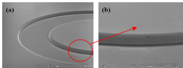
Fig. 10 SEM picture of the nickel vibration plate (a) and close-up view of the circular bulge (b)
