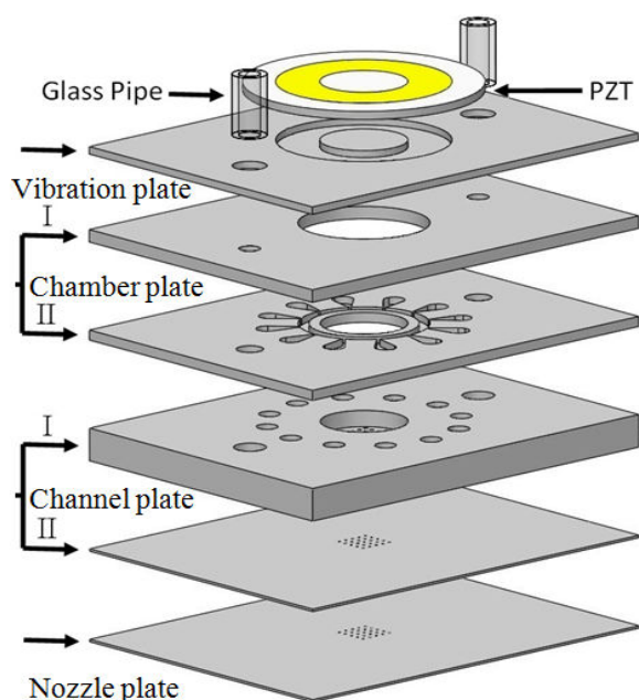
Fig. 2 Schematic of the microdroplet ejector
