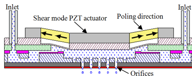
Fig. 3 The cross section view for the microdroplet ejector
