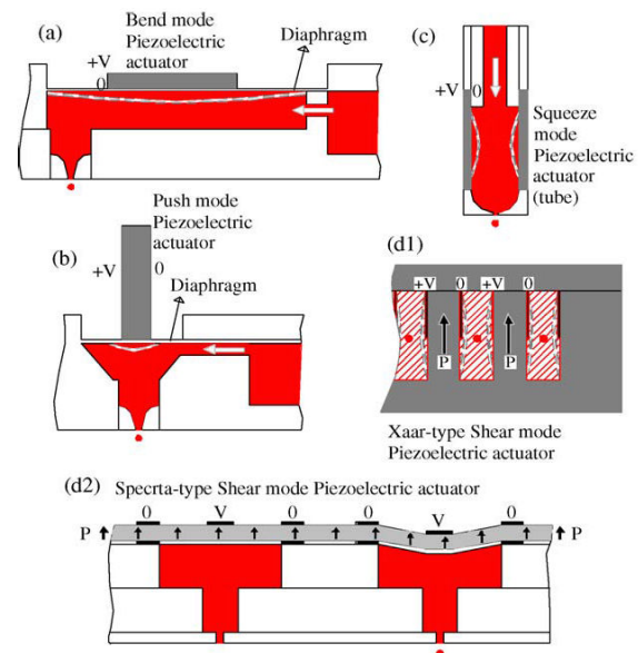
Fig. 1 Various deformation modes of piezoelectric actuators for inkjet printing technology
